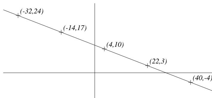
Figure 1: Graph of 7x + 18y = 208
